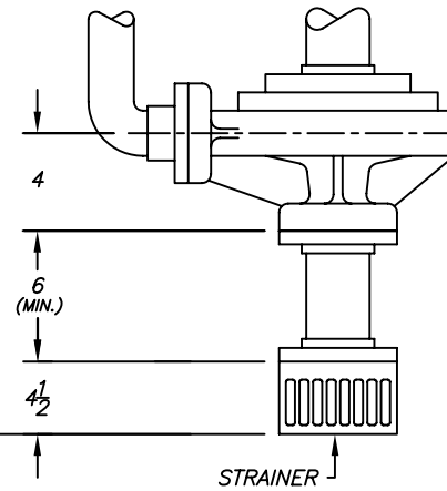
TAILPIPE ASSEMBLY (OPTIONAL)
